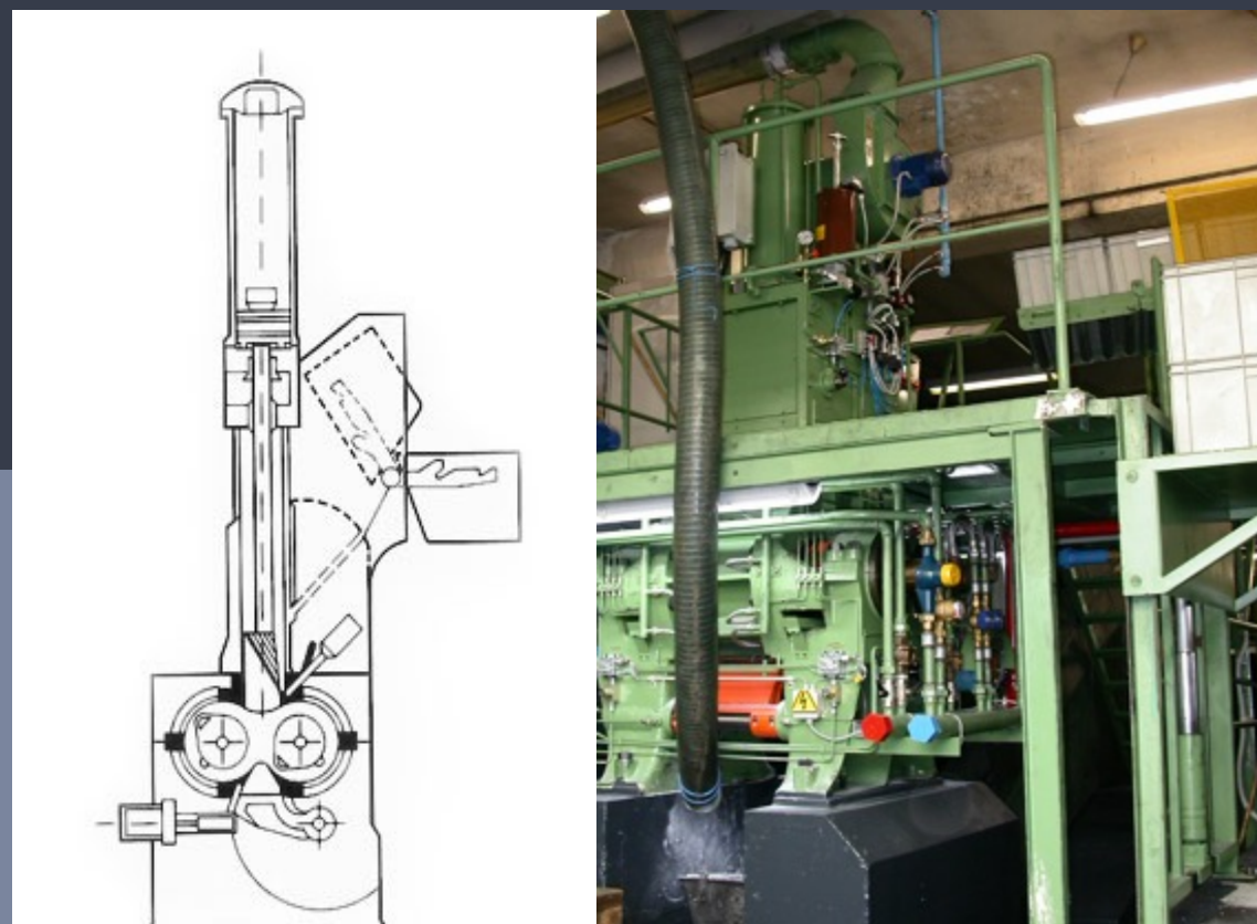
Mixing - internal mixer
